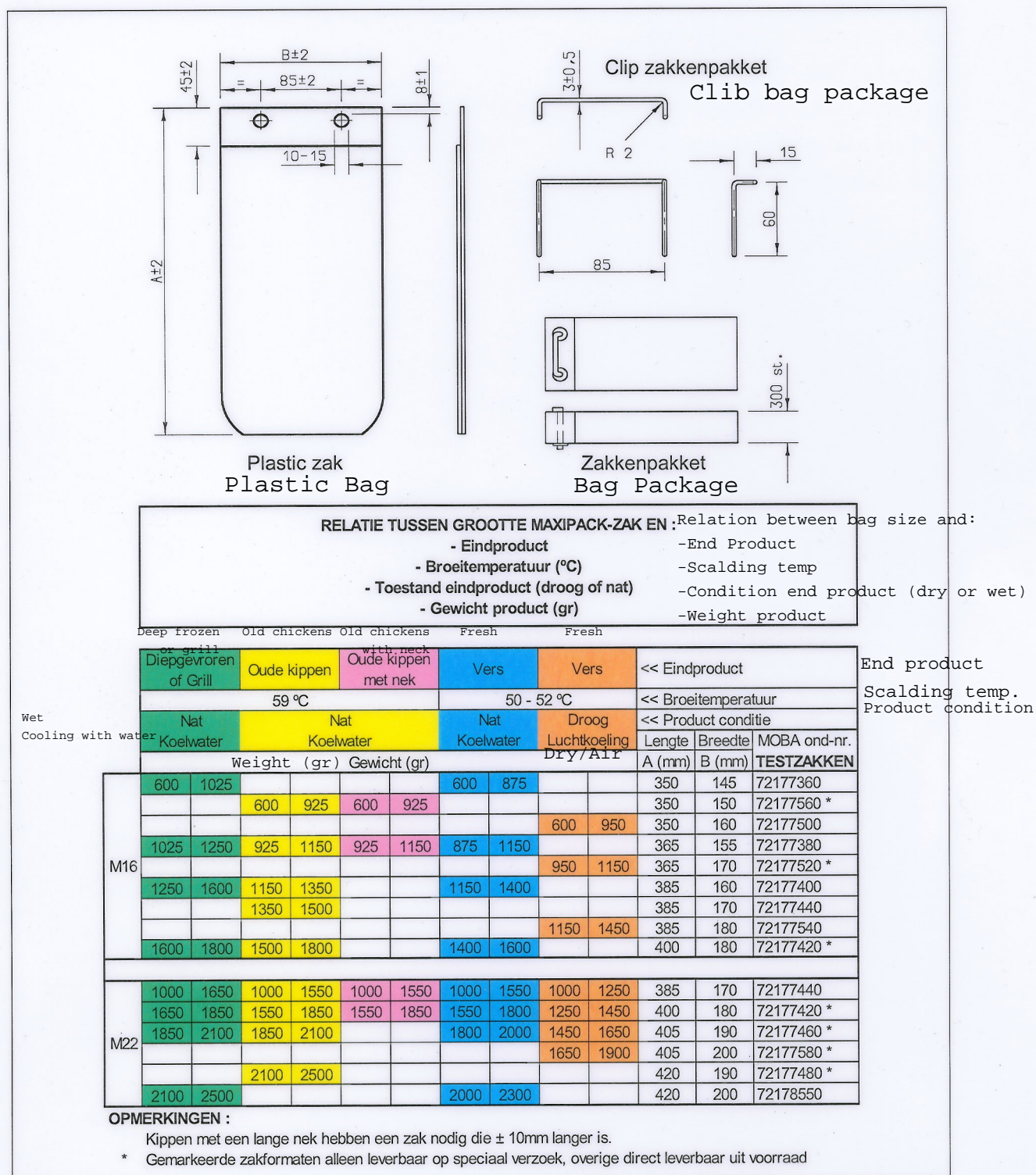
Fig. 1 - Plastic zak met clip Chickens with a long neck need a bag which is +/- 10mm longer * marked bag sizes are only available on request. Others from stock
